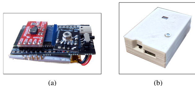
Figure 1: The developed device with pulse oximeter and IR thermometer (a), and the same device inside a 3D printed case (b).
